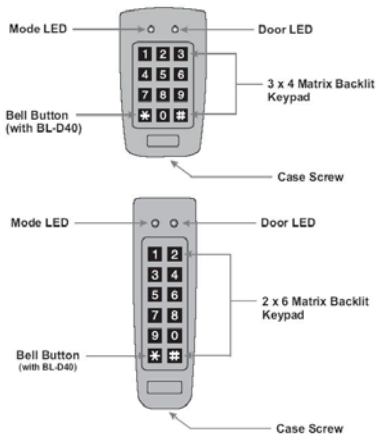
Figura 1: Panel Frontal
